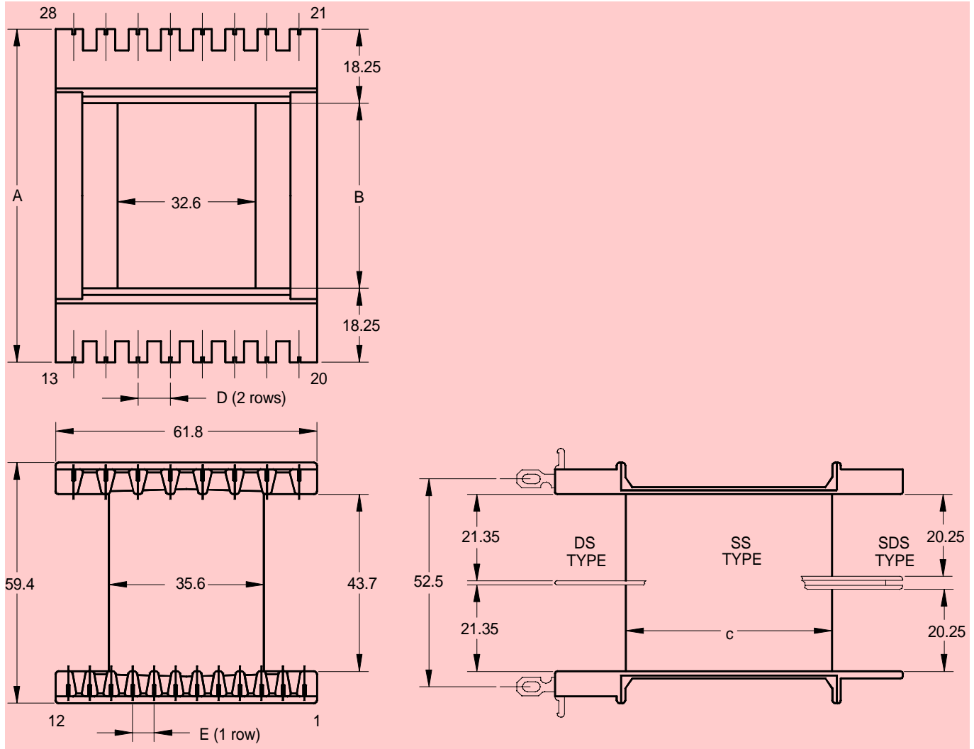
28 terminal bobbin – 2 rows of 8 tags – 1 row of 12 tags Dimensions in millimetres
