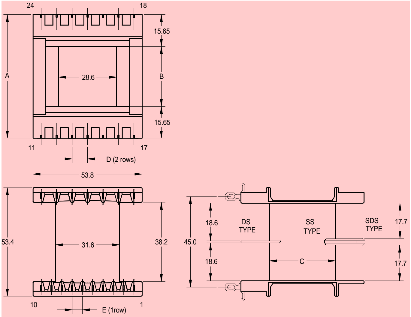
24 terminal bobbin – 2 rows of 7 tags – 1 row of 10 tags Dimensions in millimetres
