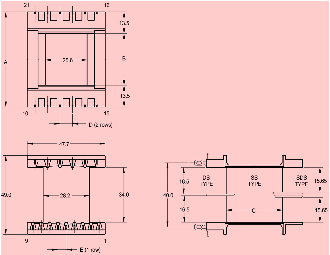
21 terminal bobbin – 2 rows of 6 tags – 1 row of 9 tags Dimensions in millimetres
