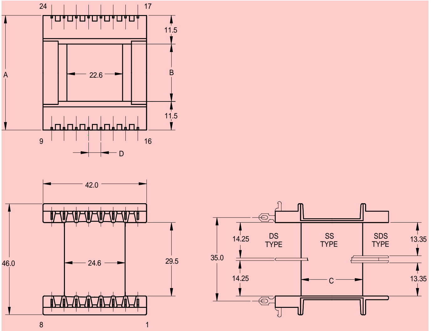
24 terminal bobbin – 3 rows of 8 tags Dimensions in millimetres
